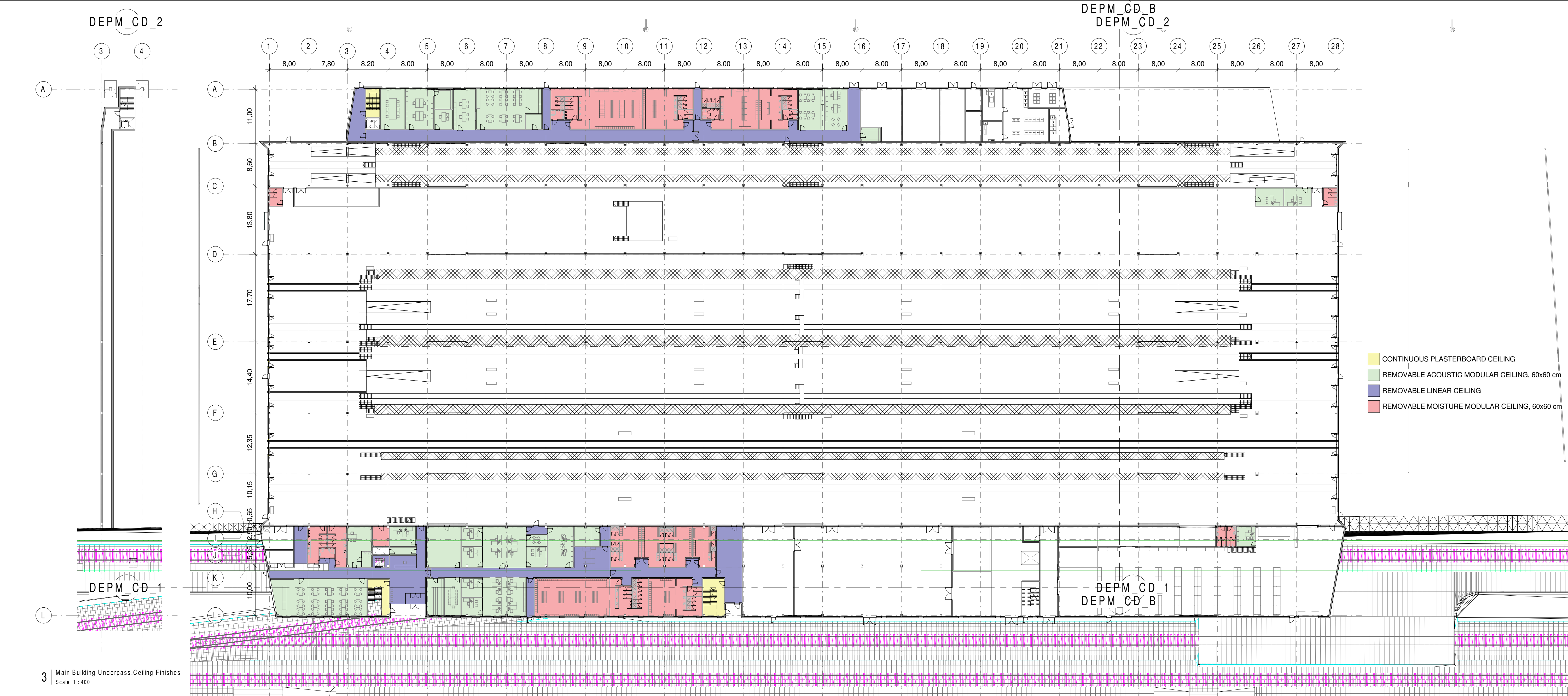
1 Main Building Ground Floor Ceiling Finishes Scale 1 : 400
